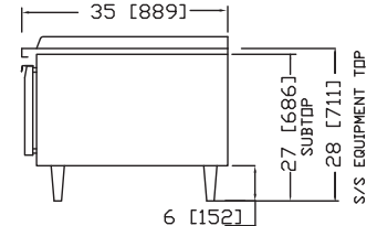
[SIDE] - "T" MODEL
